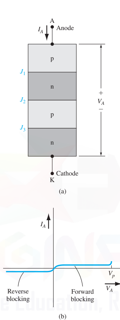
Figure 15.29 | (a) The basic four-layer pnpn structure. (b) The initial current–voltage characteristic of the pnpn device.
