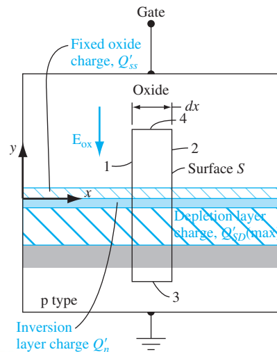
Figure 10.45 | Geometry for applying Gauss's law.
