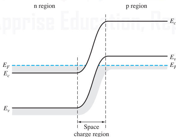
Figure 8.27 | Energy-band diagram of a pn junction in thermal equilibrium in which both the n and p regions are degenerately doped.
