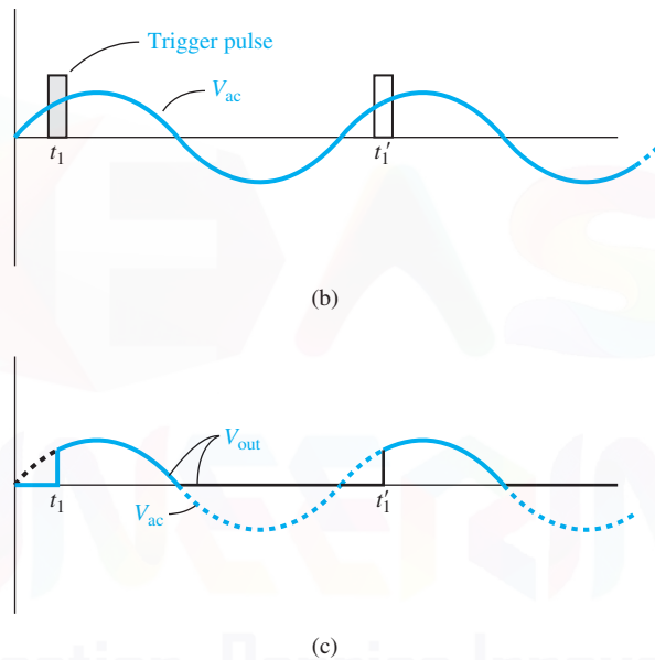
Figure 15.35 | (a) Simple SCR circuit. (b) Input ac voltage signal and trigger pulse. (c) Output voltage versus time.
