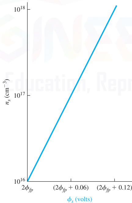
Figure 10.12 | Electron inversion charge density as a function of surface potential.
