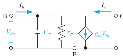
Figure 12.41 | Simplified hybrid-pi equivalent circuit.
