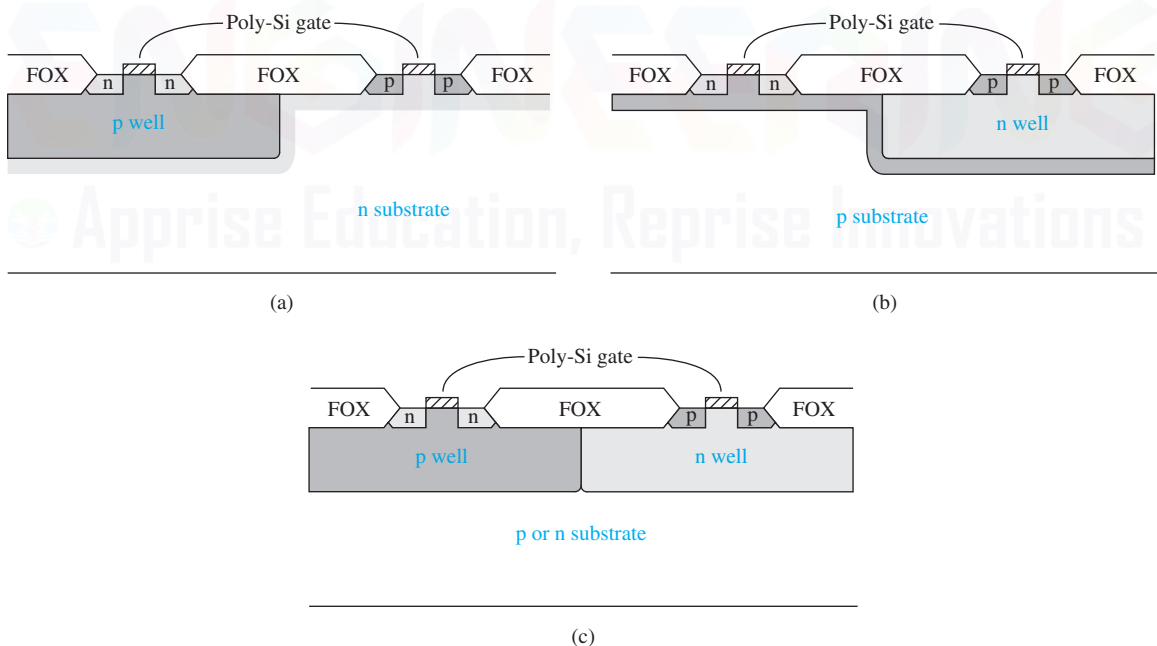
Figure 10.58 | CMOS structures: (a) p well, (b) n well, and (c) twin well.
