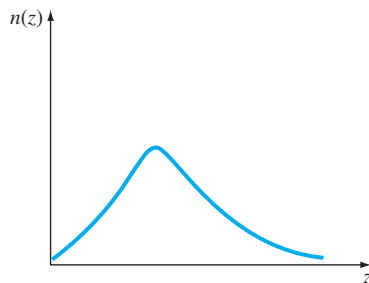
Figure 9.21 | Electron density in triangular potential well.
