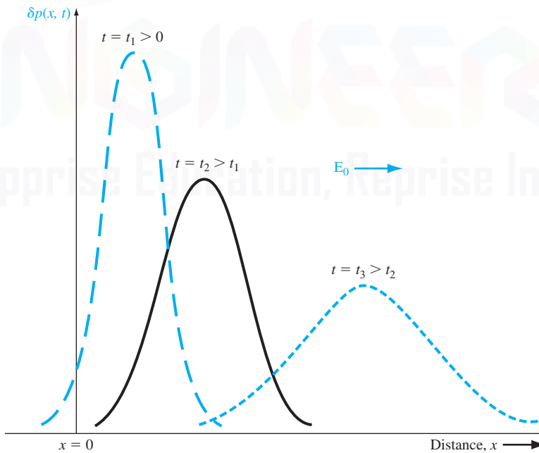
Figure 6.9 | Excess hole concentration versus distance at various times for a constant applied electric field.
