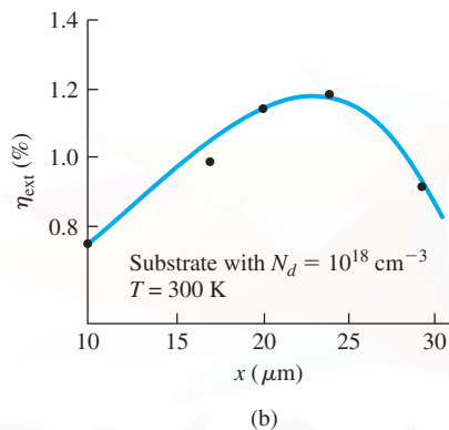
Figure 14.28 | (a) External quantum efficiency of a GaP LED versus acceptor doping. (b) External quantum efficiency of a GaAs LED versus junction depth. (From Yang [22].)
