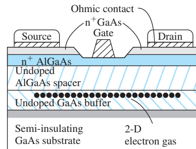
Figure 13.26 | A “normal” AlGaAs–GaAs HEMT.
